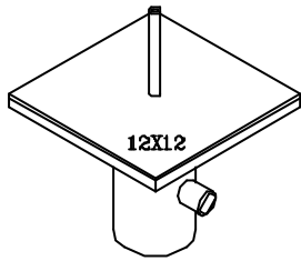
ABHPN - 8511 (QP-S-12) I.D. = \phi 0.4 O.D. = \phi 0.7
