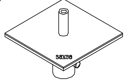
ABHPN - 8553 (QP-M-38) I.D. = \phi 1.7 O.D. = \phi 2.5
